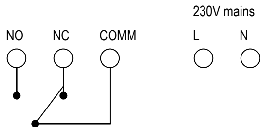
Figure 2 – ASR-RF Unit Pin Out (Rear View)
